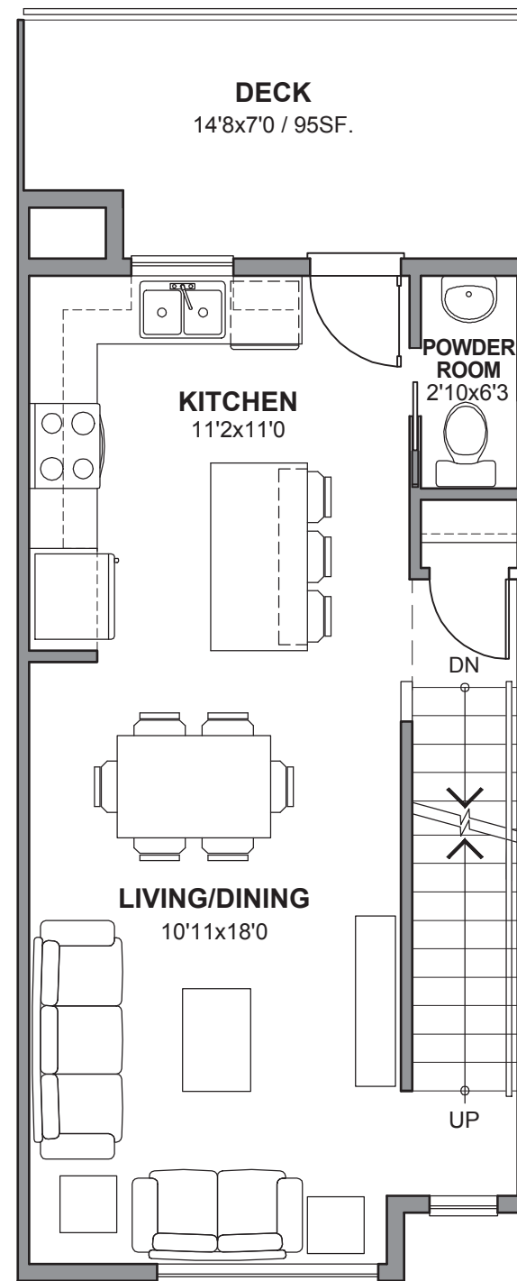
MAIN FLOOR PLAN - UNIT 'A'
