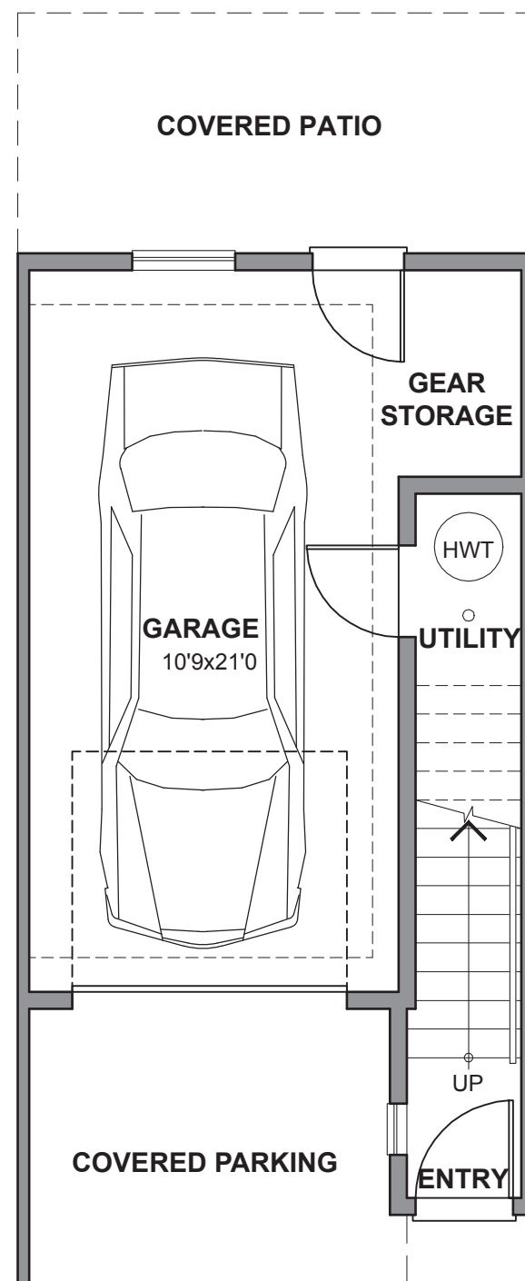
LOWER FLOOR PLAN - UNIT 'A'
